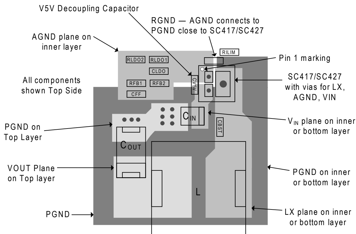
Figure 15 — PCB Layout
