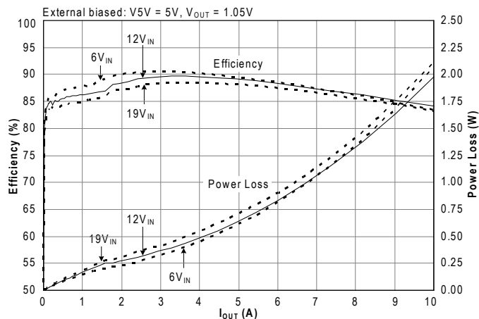
SC427 Efficiency/Power Loss vs. Load — PSAVE Mode
