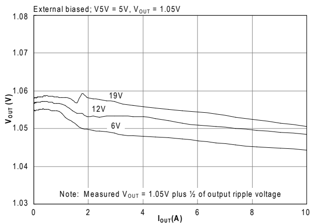
SC427 Load Regulation —PSAVE Mode
