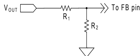
Figure 3 — Output Voltage Selection
